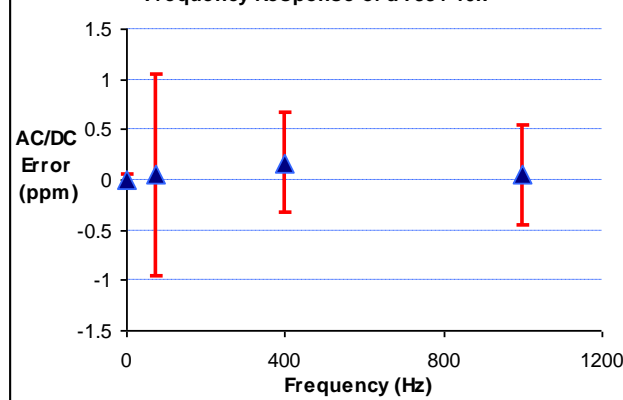
AC/DC error of a 7334- 100\text{ }\Omega and a 7334- 10\text{ k}\Omega , calibrated by the UK National Physical Laboratory (NPL)
